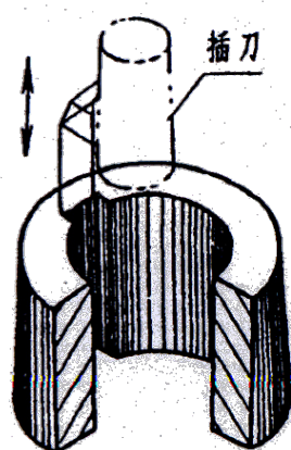
(a) 轮载上键槽
