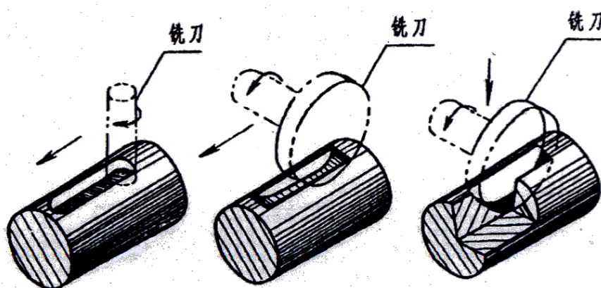
(b) 轴上键槽
