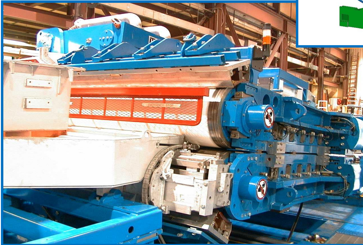
Hazelett 双带连铸机实物图
