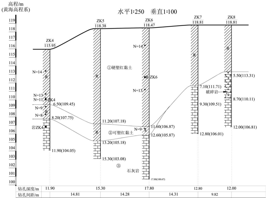
(a)地质剖面图 2-2'
