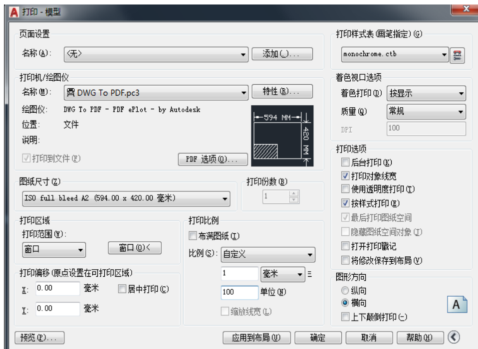
“打印”对话框
