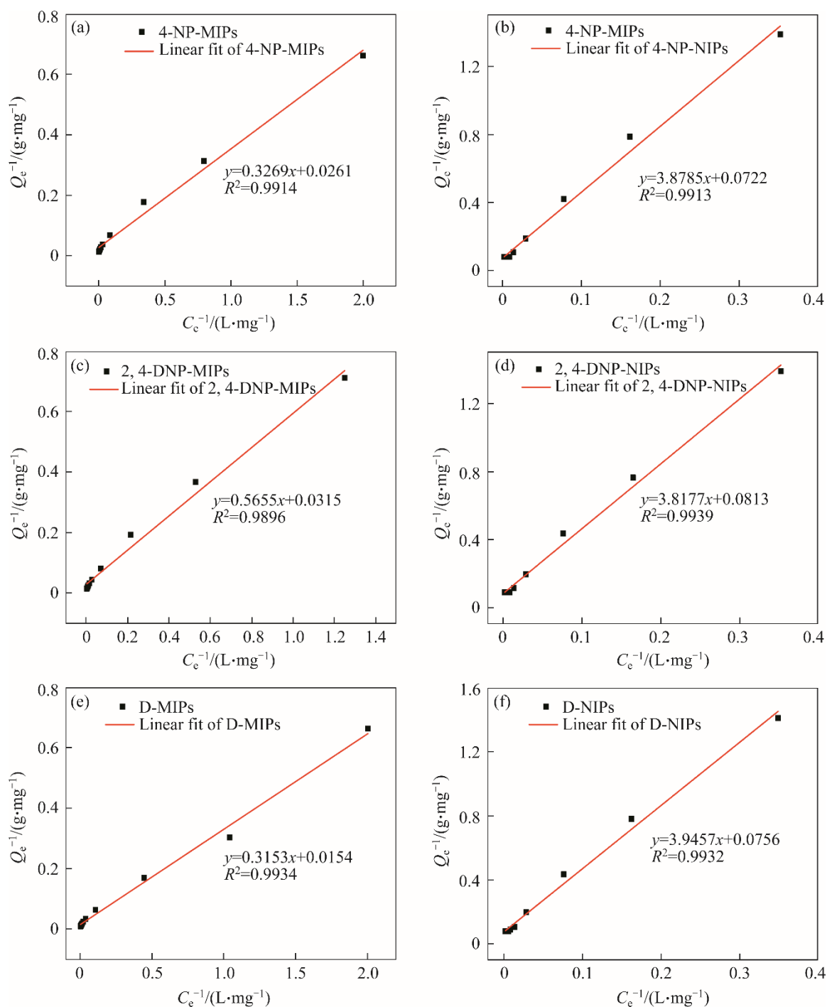
Figure S1 Langmuir model fit of MIPs and NIPs: (a) 4-NP-MIPs; (b) 4-NP-NIPs; (c) 2,4-DNP-MIPs; (d) 2,4-DNP-NIPs; (e) D-MIPs; (f) D-NIPs
