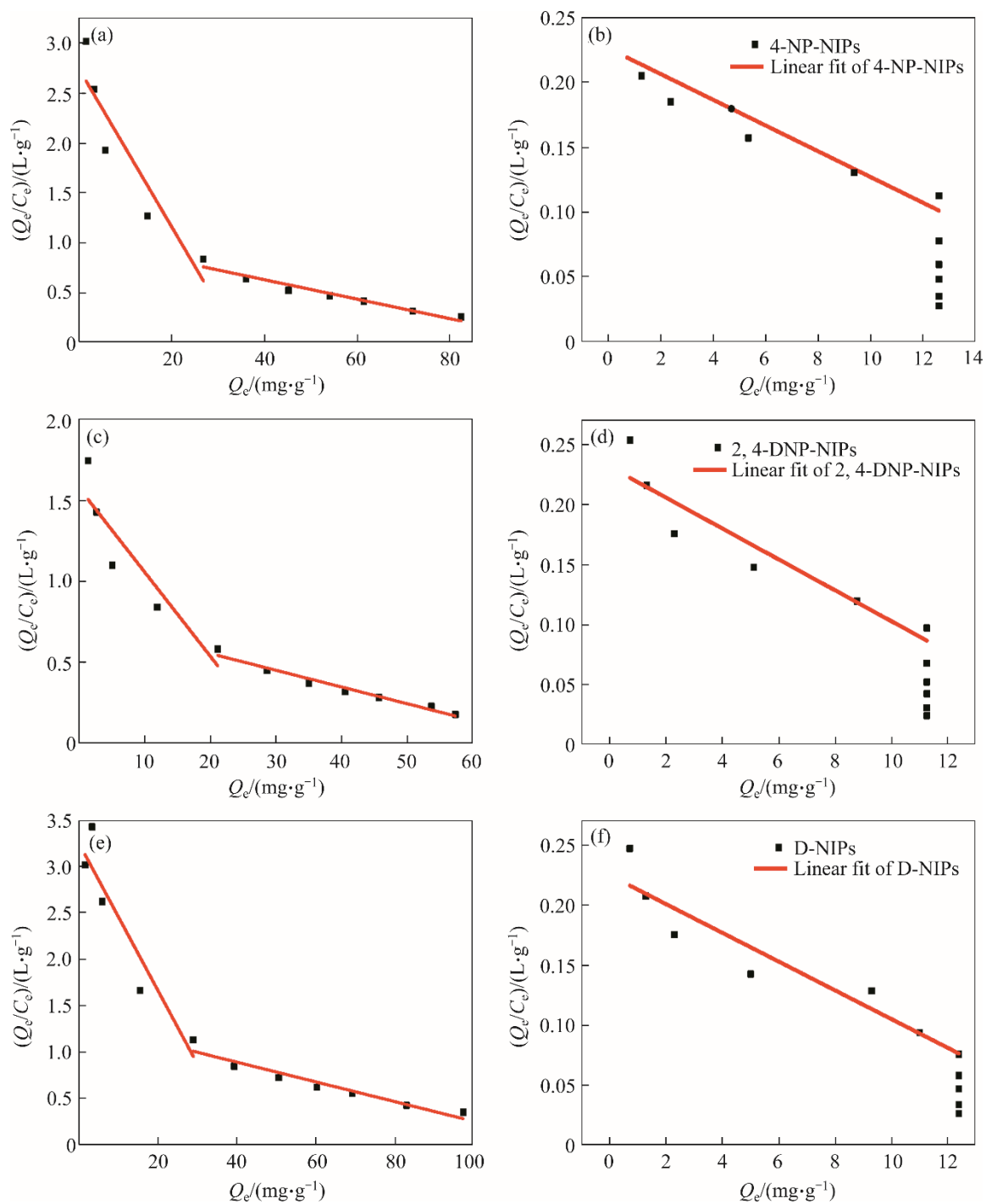
Figure S3 Scatchard fitting curves of MIPs and NIPs: (a) 4-NP-MIPs; (b) 4-NP-NIPs; (c) 2,4-DNP-MIPs; (d) 2,4-DNP-NIPs; (e) D-MIPs; (f) D-NIPs
