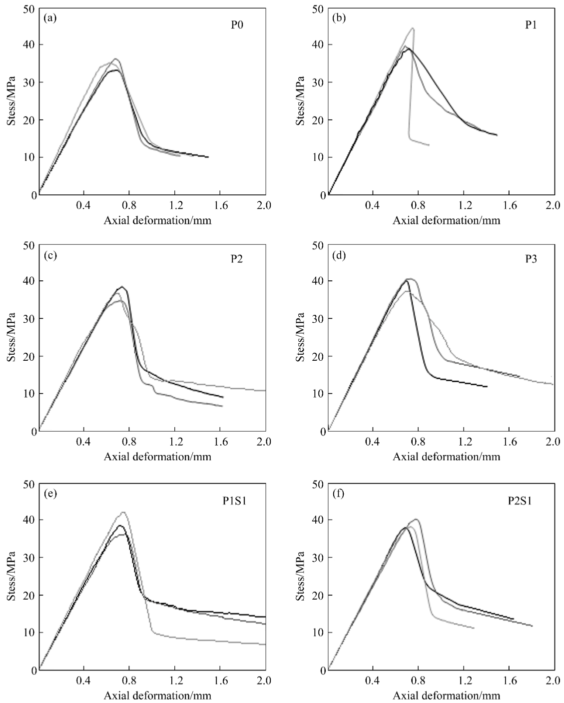
Figure S1 Stress–deformation curves of SCAC with different fiber content and fiber hybridization
