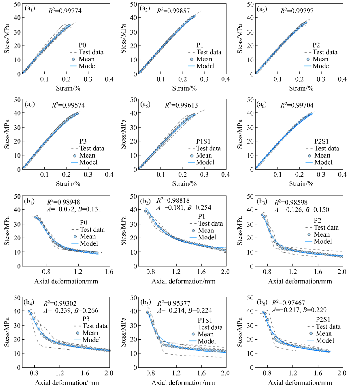
Figure S2 Comparison of modeling results and test data: (a) Prepeak stress–strain curves; (b) Postpeak stress–deformation curves
