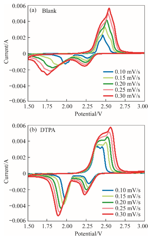
Figure S4 Cyclic voltammetry of basic electrolyte battery and 1.5 wt.% DTPA-containing electrolyte battery at different scan rates
