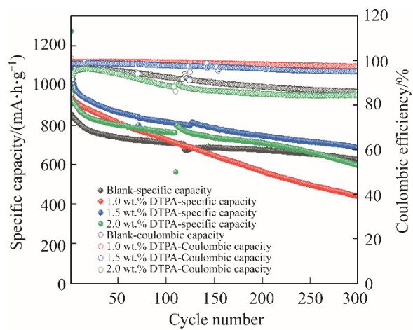
Figure S1 The cycle performance of batteries with different contents of DTPA at 0.5C
