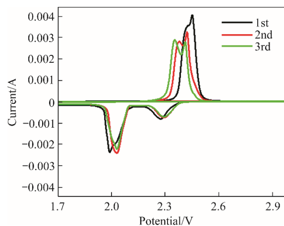
Figure S2 Cyclic voltammetry of batteries with basic electrolyte
