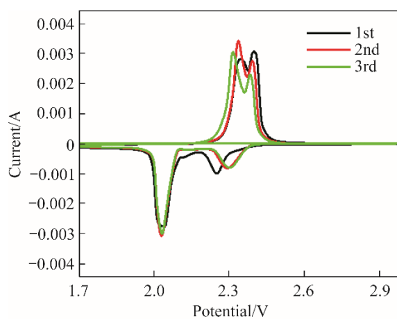
Figure S3 Cyclic voltammetry of batteries with 1.5 wt.% DTPA additive
