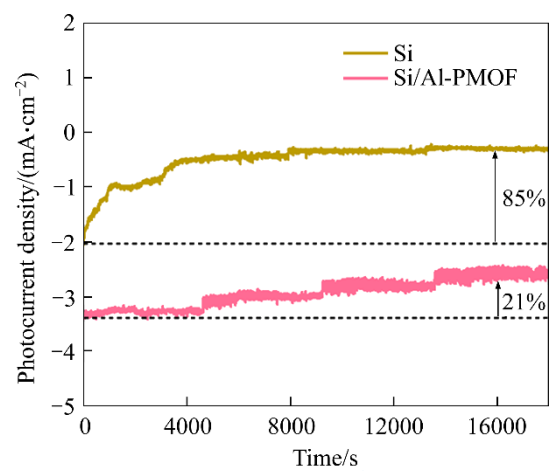
Figure S5 The stability curves of Si and Si/Al-PMOF photocathodes
