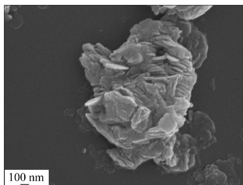
Figure S1 The SEM images of Al-PMOF
