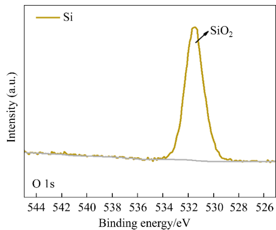
Figure S4 The high-resolution XPS spectrum of O 1s for Si photocathode
