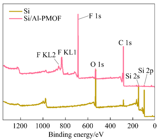
Figure S3 XPS survey of Si and Si/Al-PMOF photocathodes
