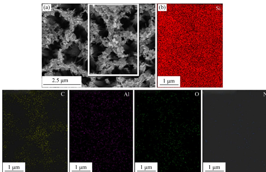
Figure S2 (a) The selected SEM image of Si/Al-PMOF photocathode; (b) The corresponding EDS elemental maps
