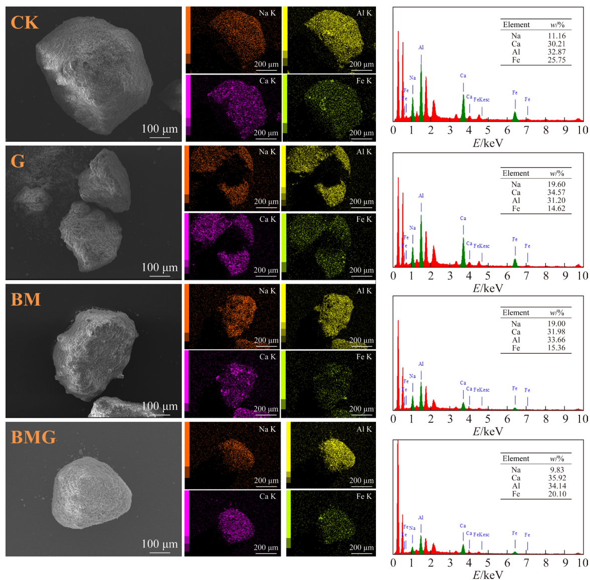
Figure S2 Element distribution and energy-dispersive X-ray analysis of bauxite residue after 180-d incubation
