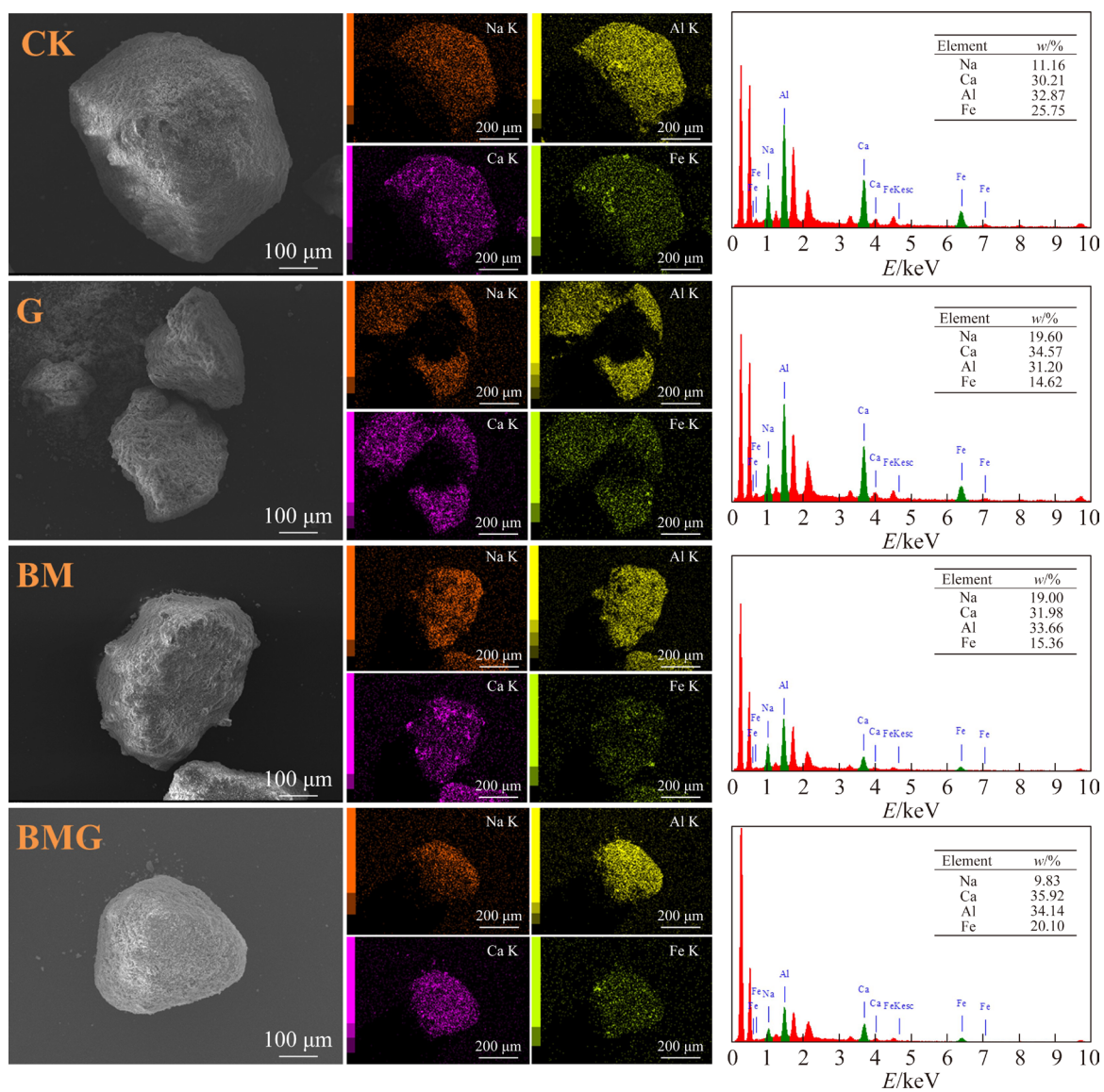
Figure S1 Element distribution and energy-dispersive X-ray analysis of bauxite residue after 60-d incubation
