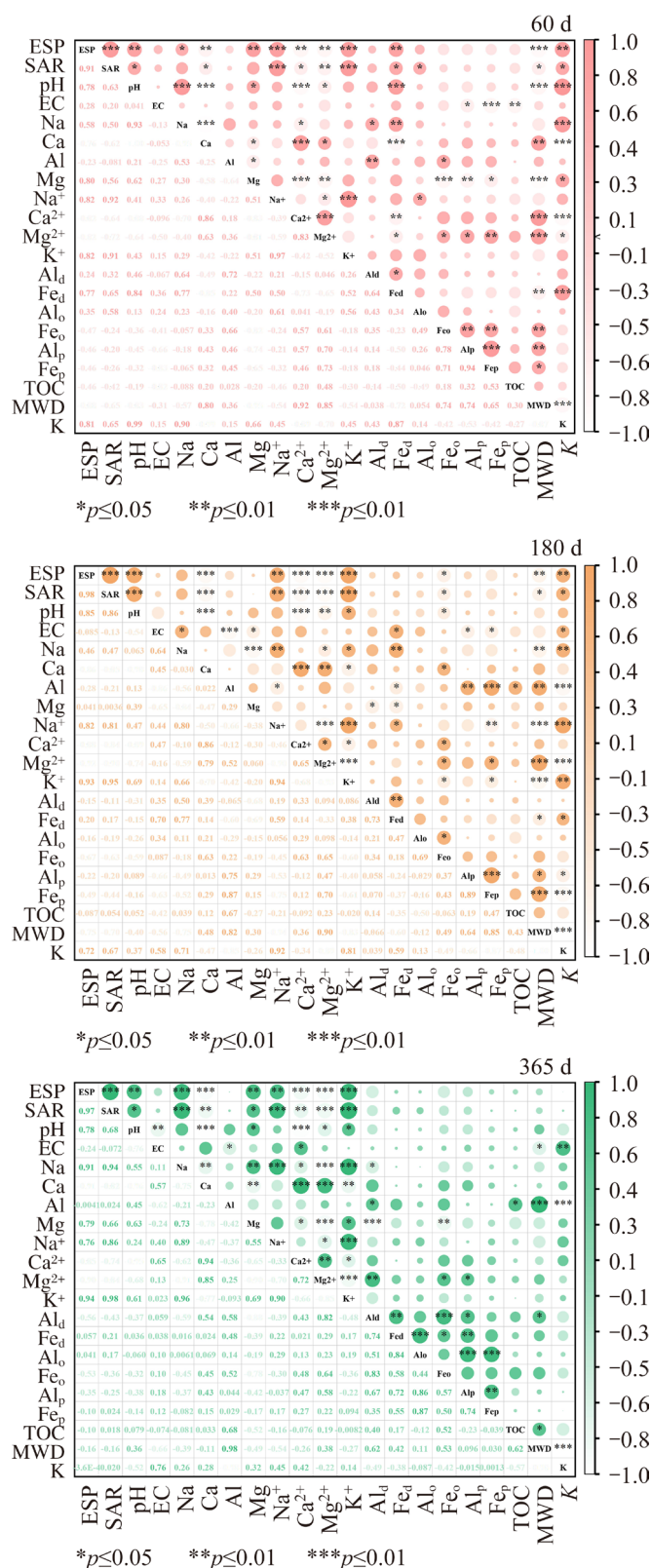
Figure S3 Pearson correlation analysis between the residue properties and aggregate stability of bauxite residue over time
