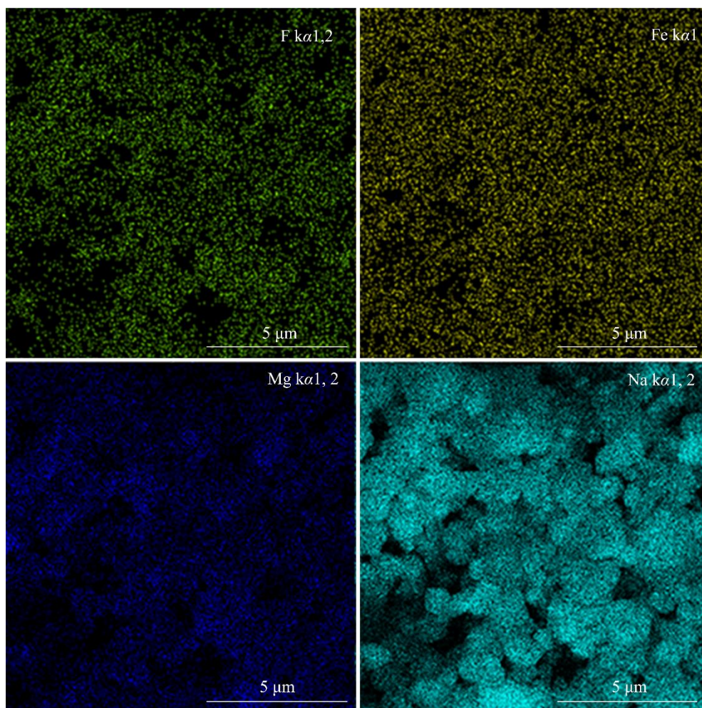
Figure S1 SEM-EDS analysis of heavy metal gypsum residue
