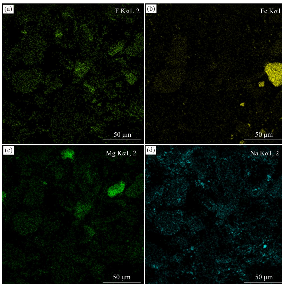
Figure S2 SEM-EDS analysis of zinc - containing fume
